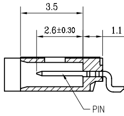
SECT. Y-Y
